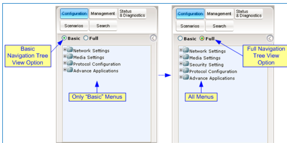
Figure 4-1: Web Interface Showing Basic/Full Navigation Tree Display
