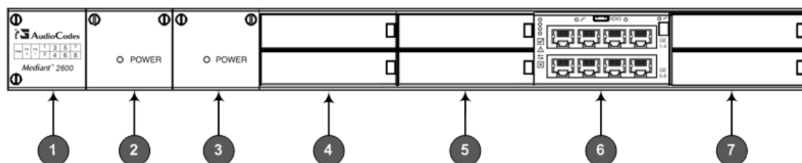
Figure 3-1: Front Panel
