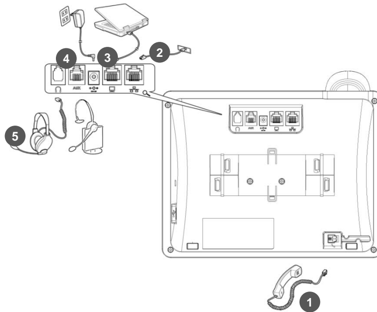
Figure 2-3: Cabling
