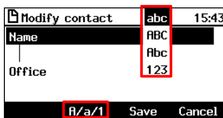
Figure 3-3: Alphanumerical Selection
