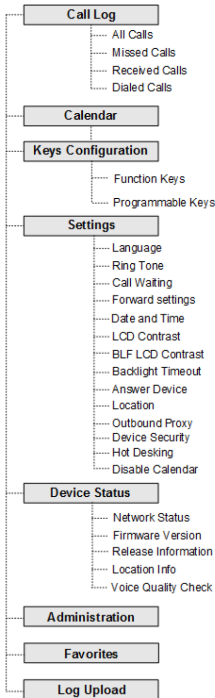
Figure 3-2: Phone Menu
