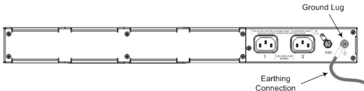
Figure 5-1: Grounding the Device
