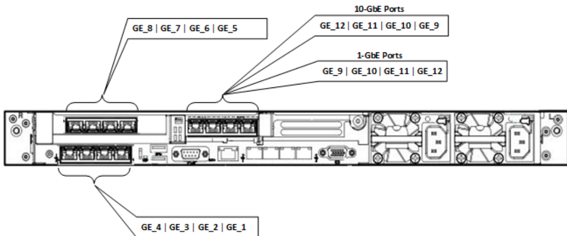
Figure 13-2: Mediant 9080 / Mediant 9000 Rev. B Ethernet Port String Names
