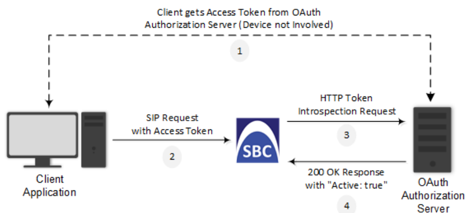
Figure 22-1: General Stages of OAuth-based Authentication
