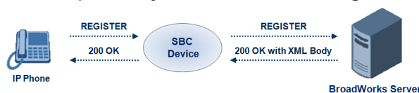
Figure 37-4: Interoperability with BroadWorks Registration Process
