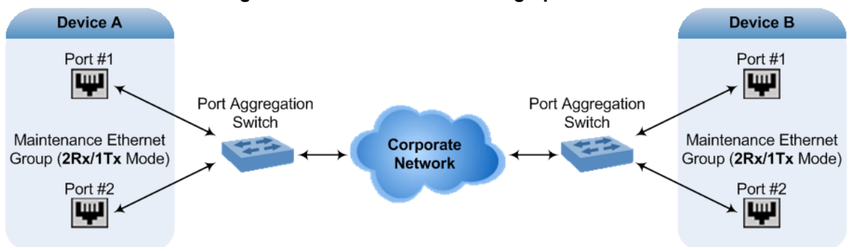
Figure 41-3: Rx/Tx Mode for Geographical HA
