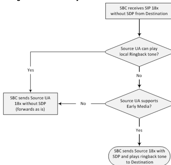
Figure 28-7: SBC Early Media RTP 18x without SDP
