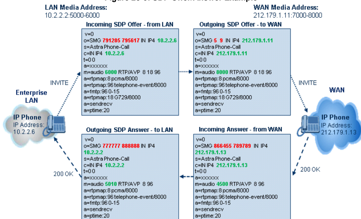
Figure 28-3: SDP Offer/Answer Example
