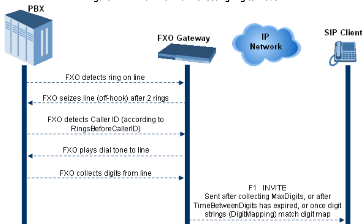
Figure 27-11: Call Flow for Collecting Digits Mode
