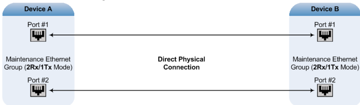
Figure 41-1: Rx/Tx Mode for Direct Connection
