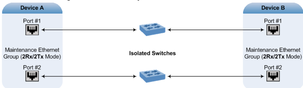
Figure 41-2: Redundancy Mode for Two Isolated Switches
