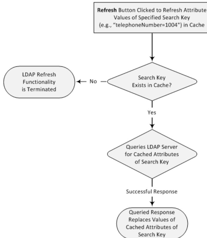
Figure 15-19: LDAP Cache Refresh Flowchart
