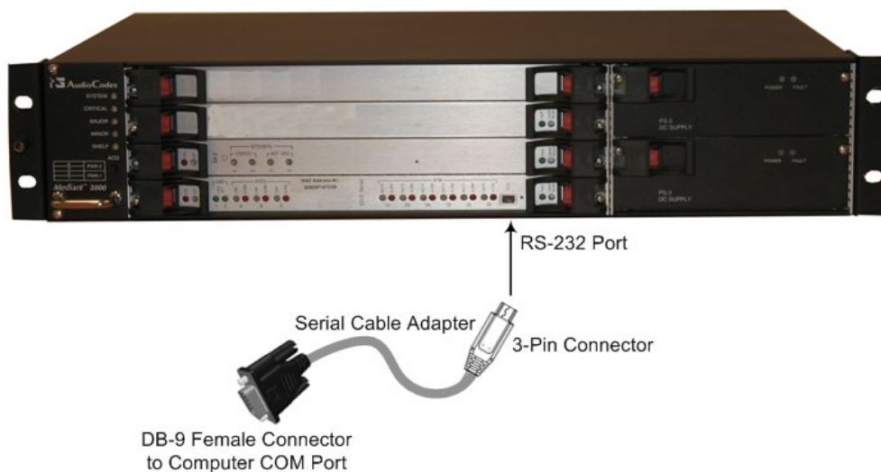
Figure 4-5: Serial Connection with PC for CLI Communication for TP-8410
