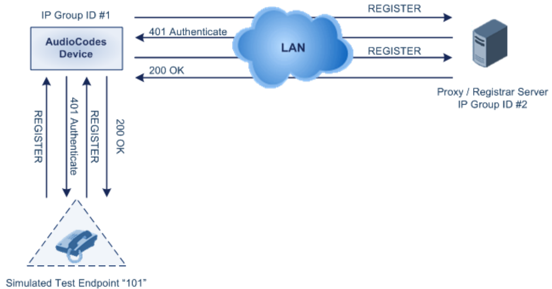
Figure 49-10: Test Call Registration Example
