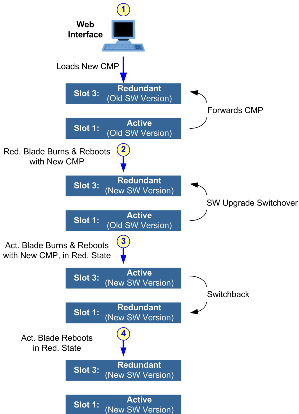
Figure 38-5: Hitless SW Upgrade Process
