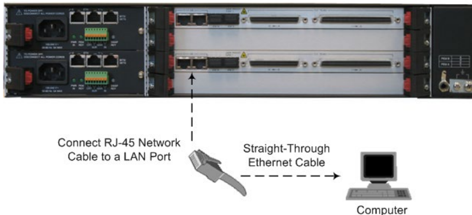
Figure 4-1: LAN Connection to PC for Initial Connectivity for RTM-8410
