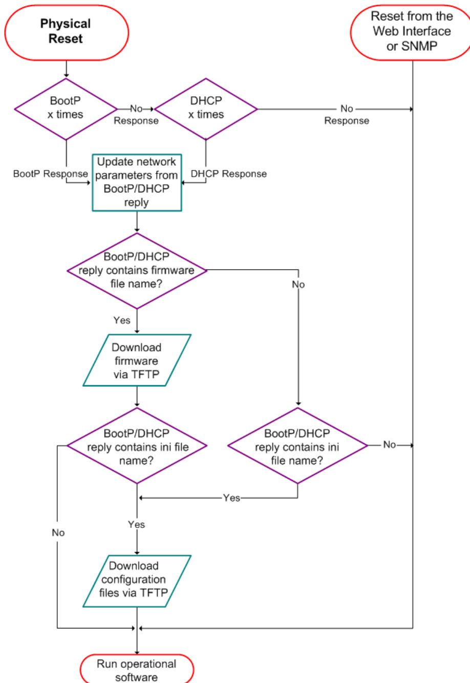
Figure 39-1: BootP Request and DHCP Discovery upon Startup
