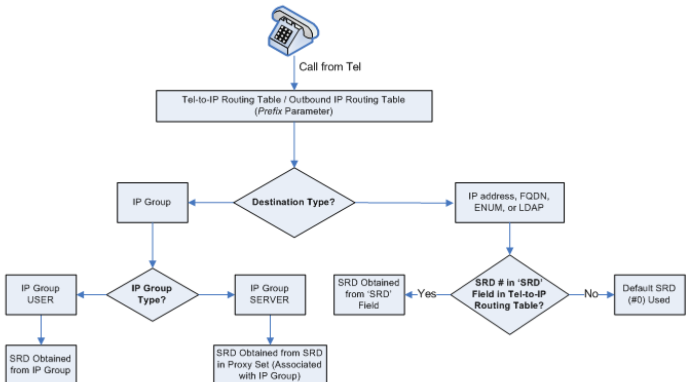
Figure 25-2: Locating SRD
