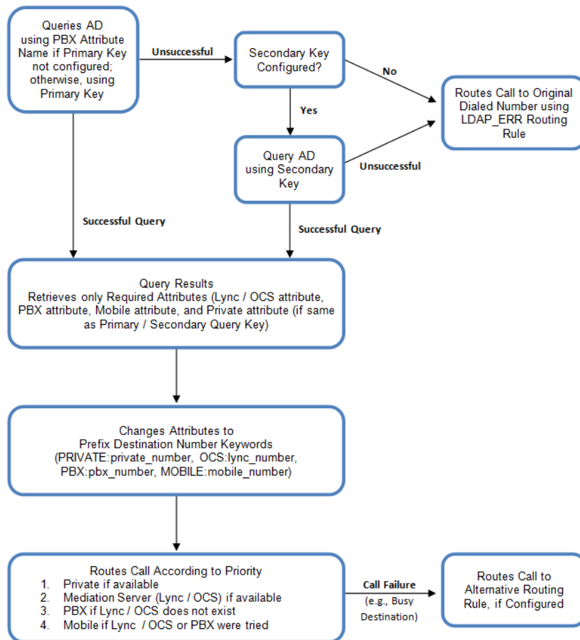
Figure 16-22: LDAP Query Flowchart
