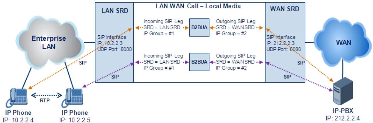
Figure 28-5: SBC SIP Signaling without RTP Media Flow
