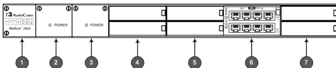
Figure 3-1: Front Panel
