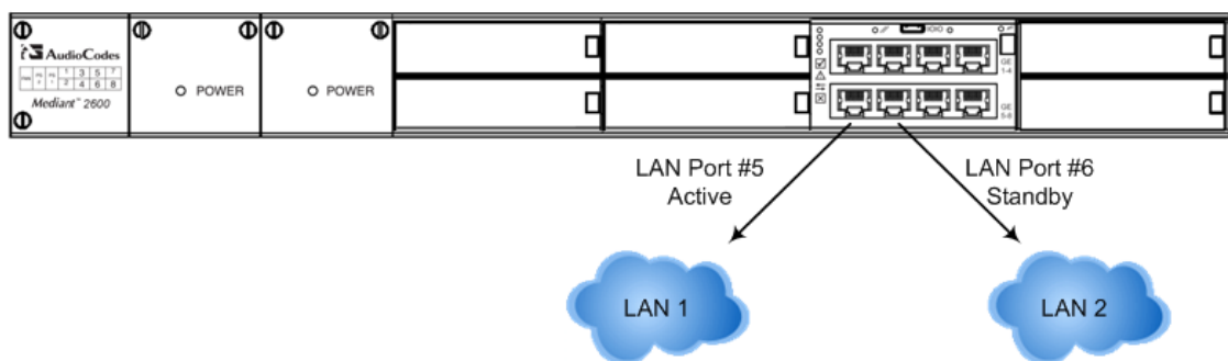
Figure 5-4: Cabling for 1+1 Ethernet-Port Redundancy (Example)
