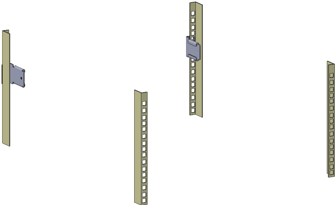
Figure 4-3: Rear-Mounting Brackets Attached to Rear-Rack Posts (> 70 cm)
