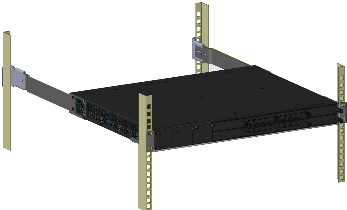
Figure 4-10: Front-Mounting Brackets Flush and Aligned with Front-Rack Posts (60 cm)
