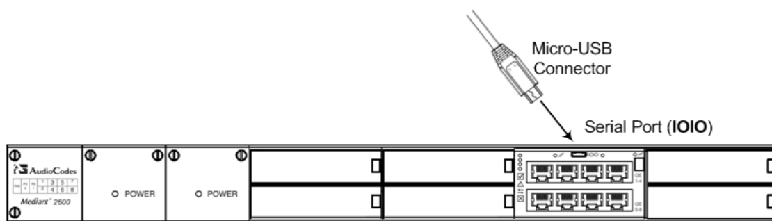
Figure 5-7: Connecting the Serial Interface
