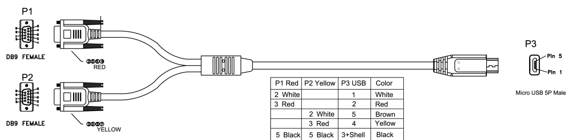
Figure 5-6: Serial Interface Cable Adapter and Connector Pinouts
