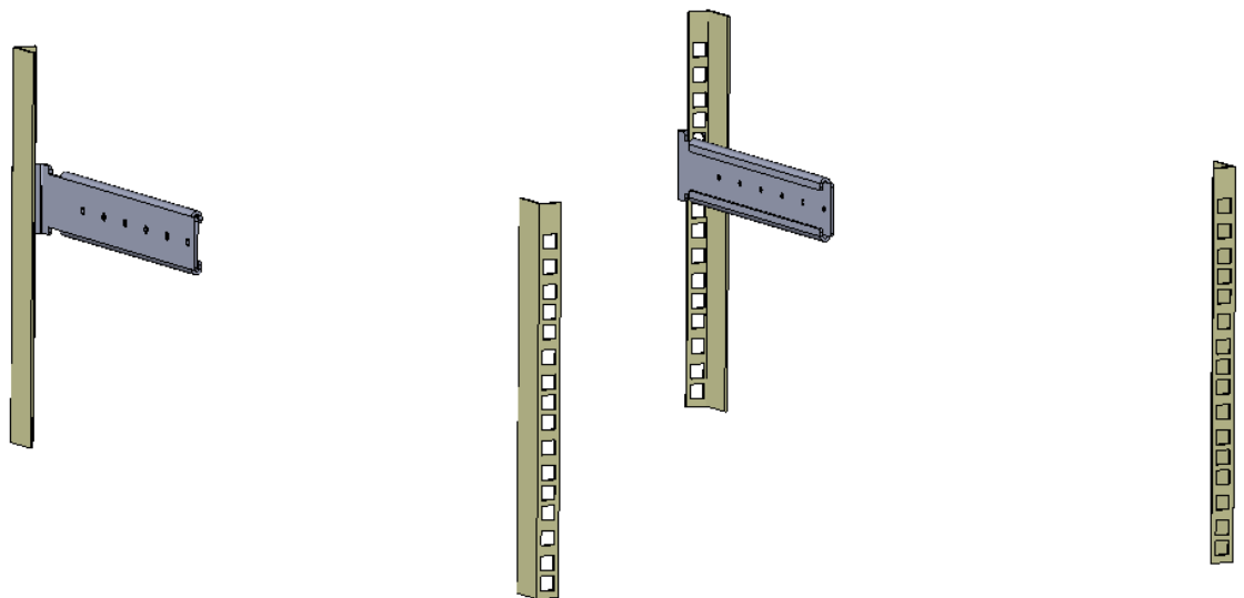
Figure 4-3: Rear-Mounting Brackets Attached to Rear-Rack Posts (> 70 cm)
