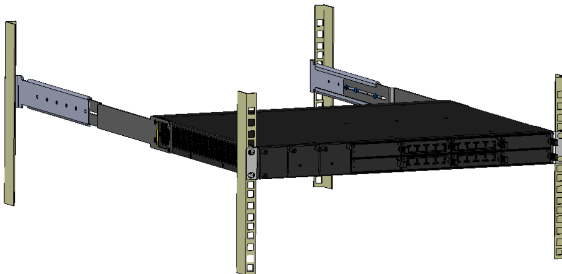
Figure 4-11: Front-Mounting Brackets Flush and Aligned with Front-Rack Posts (> 70 cm)
