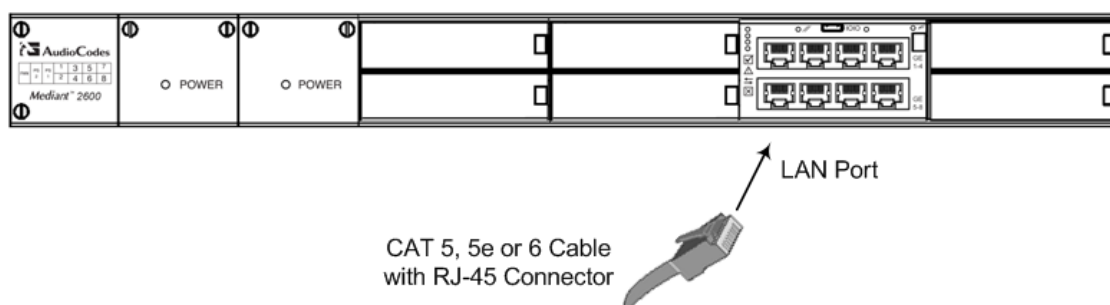
Figure 5-2: Connecting the LAN Interface
