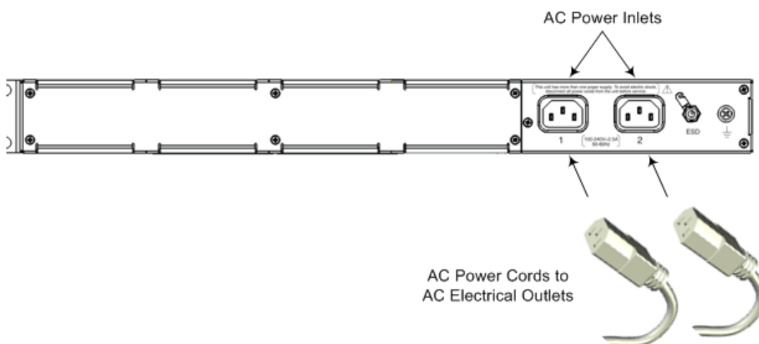
Figure 5-8: Connecting to Power
