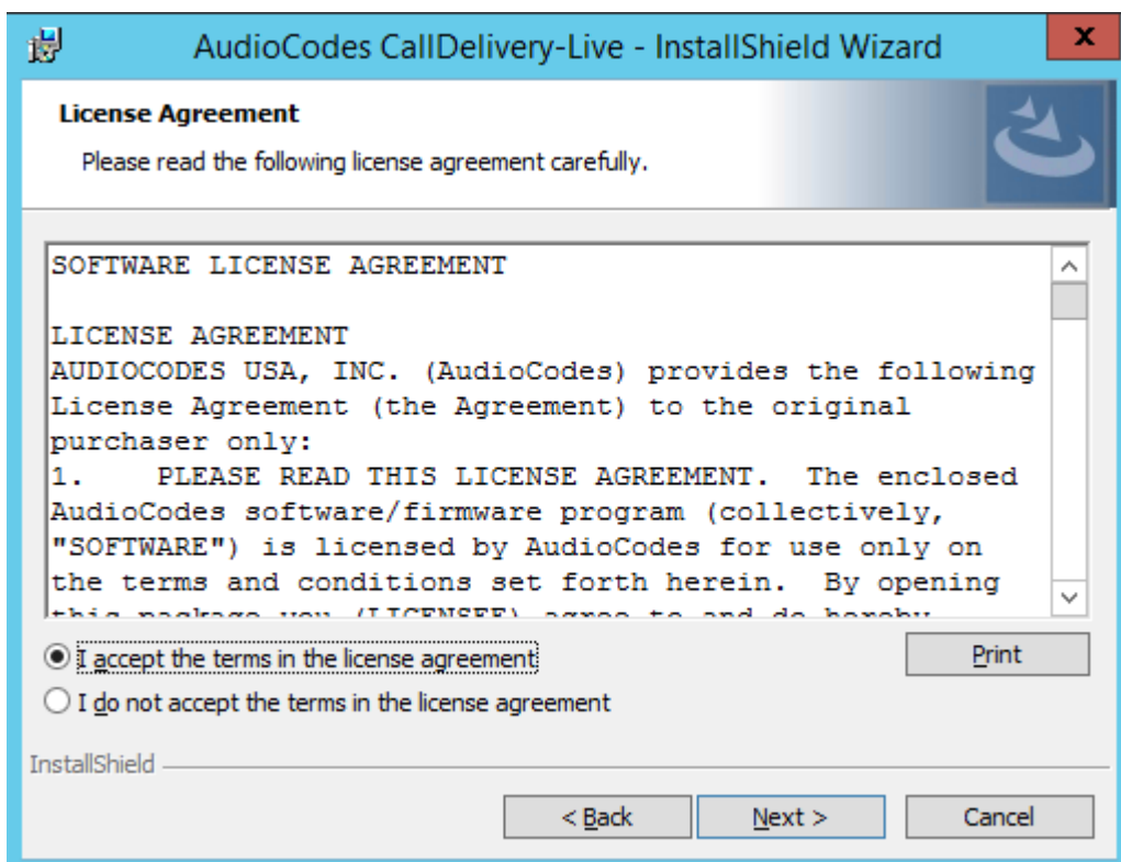
Figure 4-18: License Agreement
