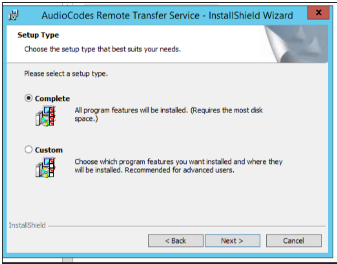
Figure 4-16: Setup Type
