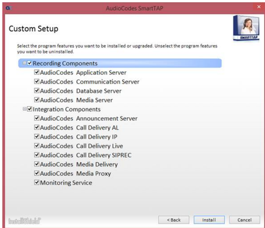
Figure 5-3: Custom Setup
