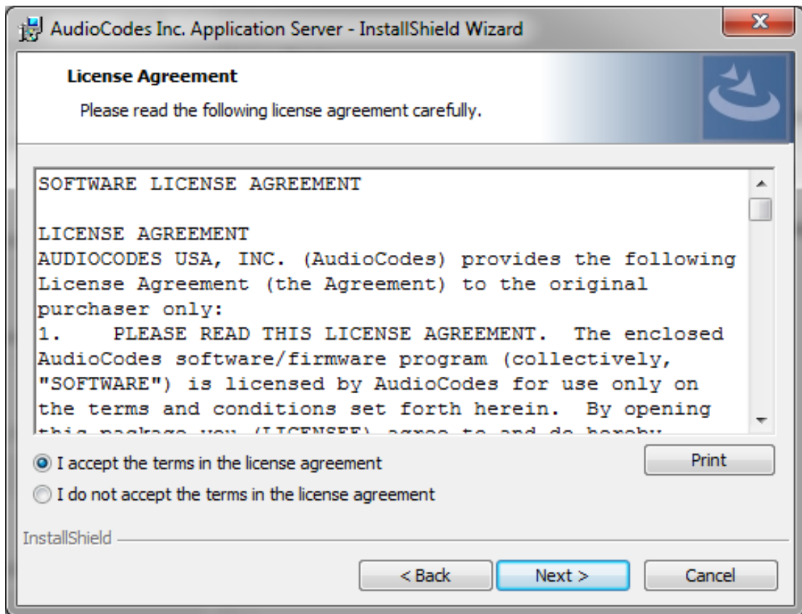
Figure 4-5: License Agreement
