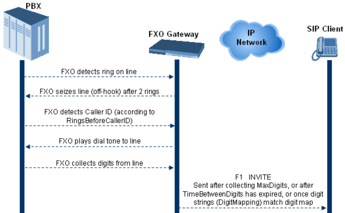
Figure 31-9: Call Flow for Collecting Digits Mode
