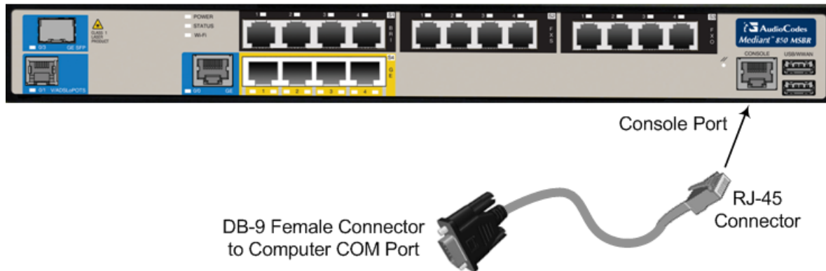
Figure 3-4: Connecting to Serial Port
