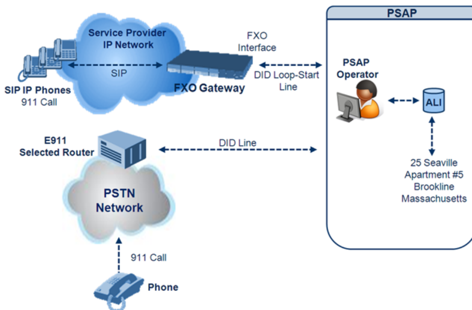
Figure 30-4: FXO Device Interfacing between E911 Switch and PSAP
