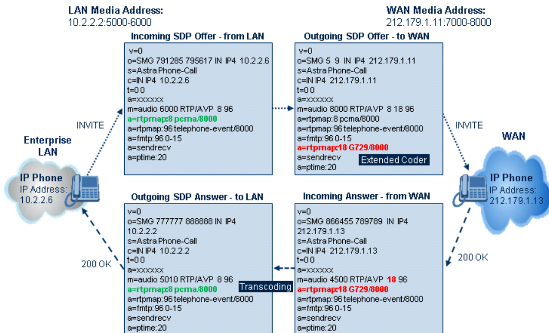
Figure 32-4: Transcoding using Extended Coders (Example)
