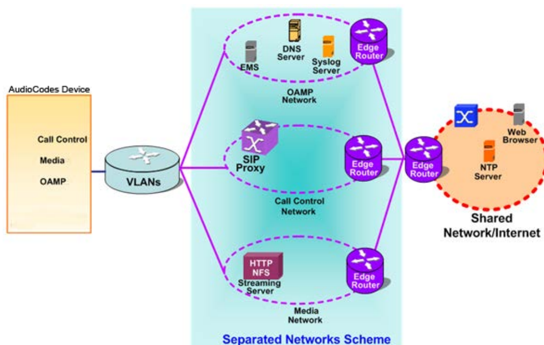
Figure 11-3: Multiple Network Interfaces
