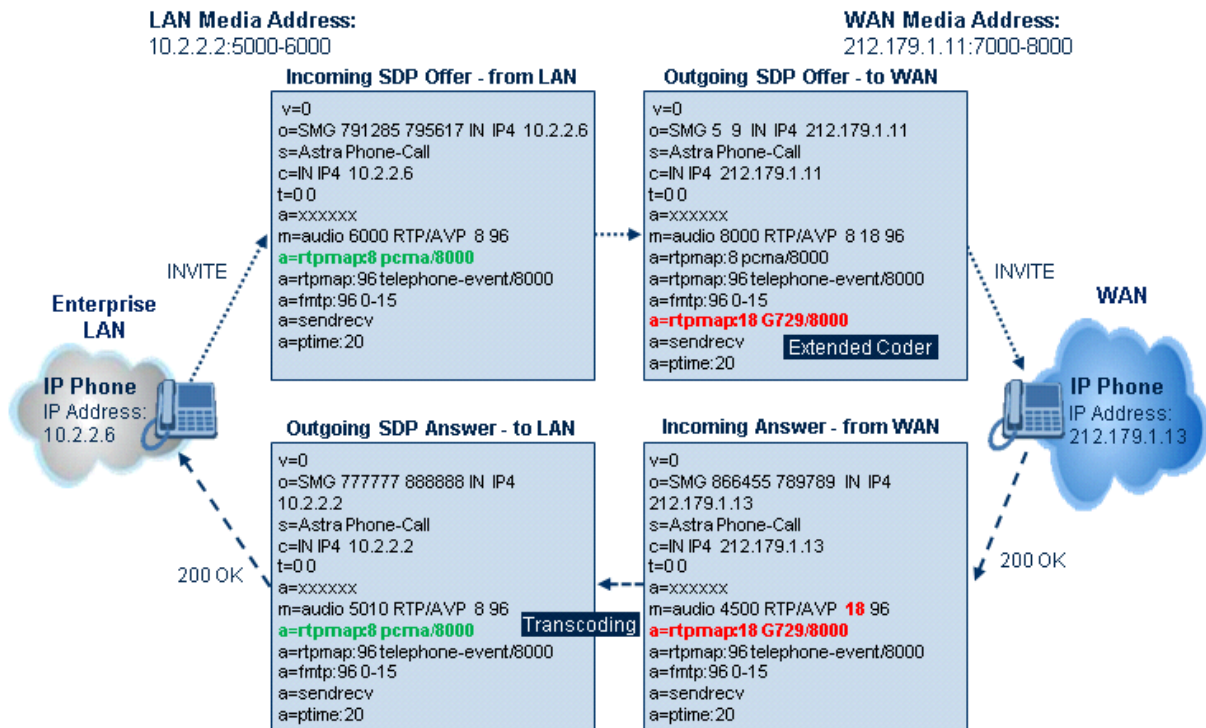
Figure 27-4: Transcoding using Extended Coders (Example)
