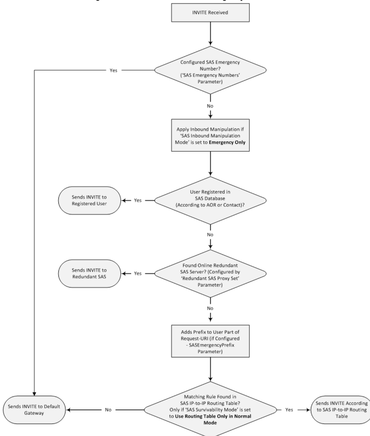
Figure 31-7: Flowchart for SAS Emergency State
