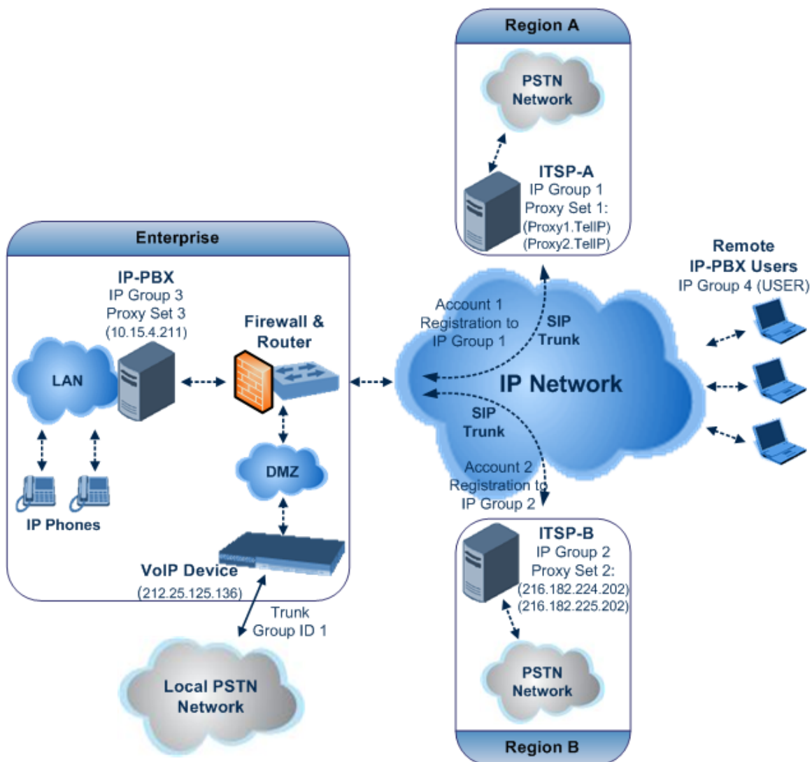
Figure 19-5: SIP Trunking Setup Scenario Example
