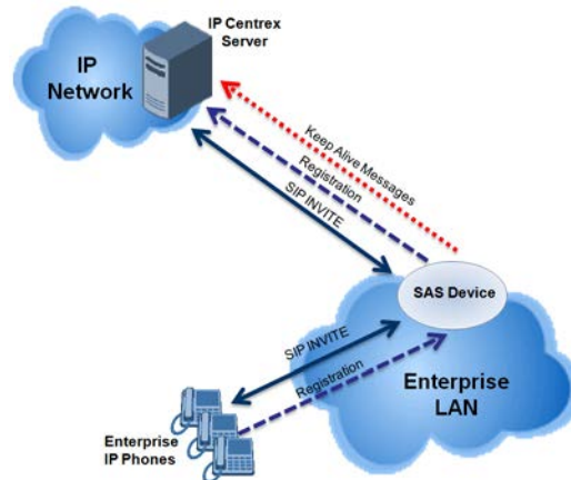
Figure 31-1: SAS Outbound Mode in Normal State (Example)
