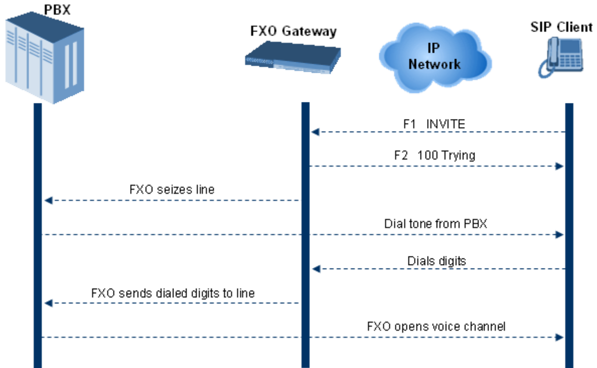
Figure 26-13: Call Flow for Two-Stage Dialing
