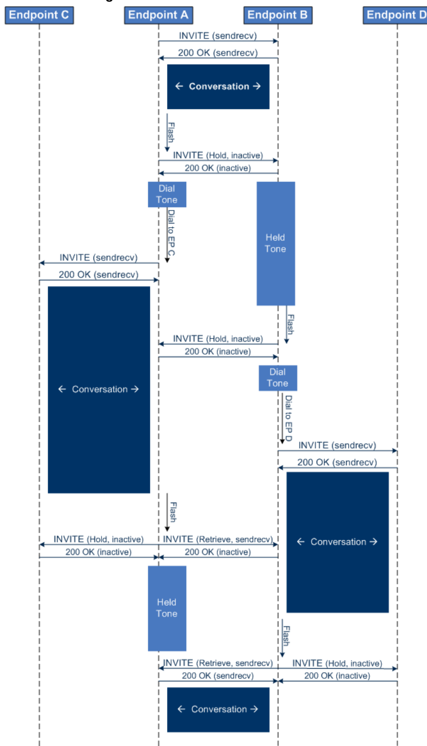
Figure 25-1: Double Hold SIP Call Flow
