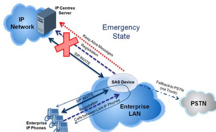
Figure 31-2: SAS Outbound Mode in Emergency State (Example)
