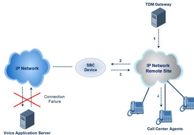
Figure 27-12: Call Survivability for Call Center
