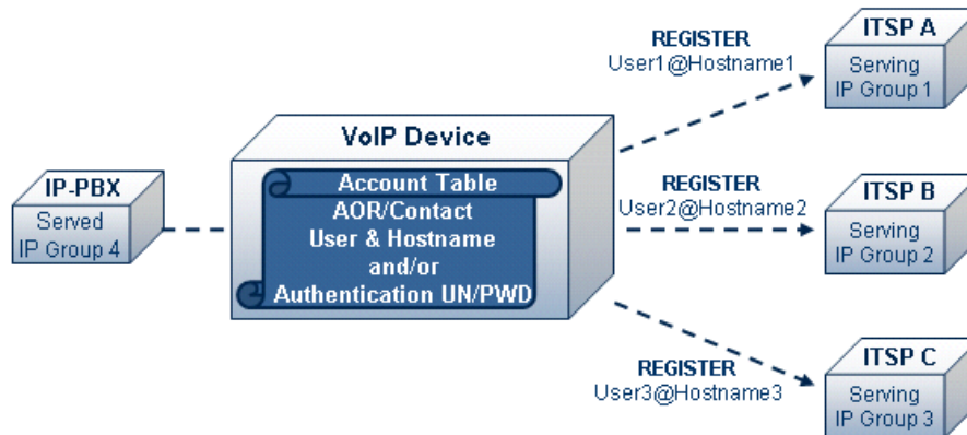
Figure 19-4: Registration with Multiple ITSP's on Behalf of IP-PBX
