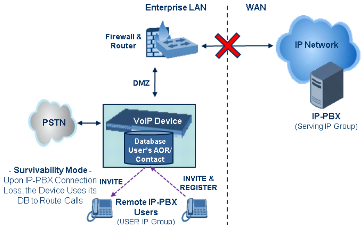
Figure 19-3: IP-to-IP Routing for IP-PBX Remote Users in Survivability Mode (Example)
