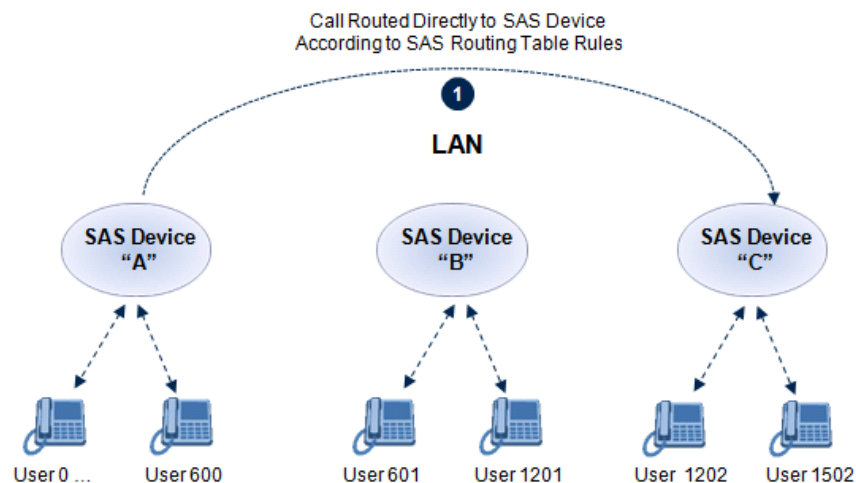
Figure 33-2: SAS Cascading Using SAS Redundancy Mode - Example
