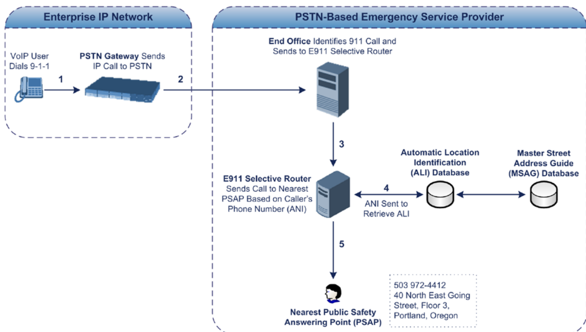
Figure 25-5: Call Flow of E9-1-1 to PSTN-Based Emergency Services Provider
