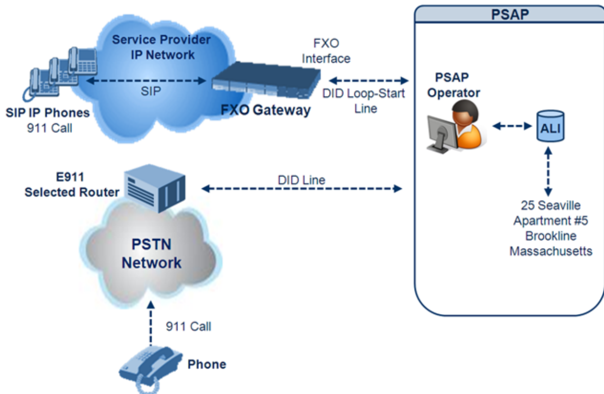
Figure 25-4: FXO Device Interfacing between E911 Switch and PSAP
