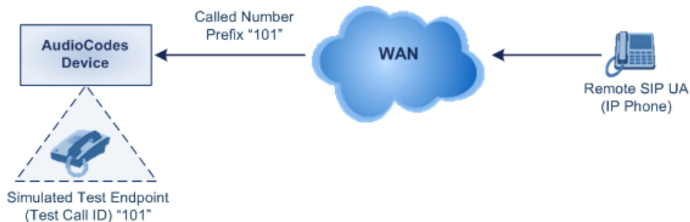
Figure 52-4: Incoming Test Call Example
