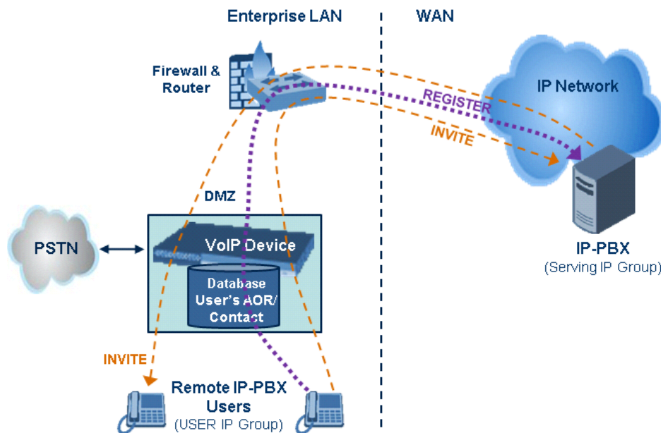
Figure 19-2: IP-to-IP Routing/Registration/Authentication of Remote IP-PBX Users (Example)
