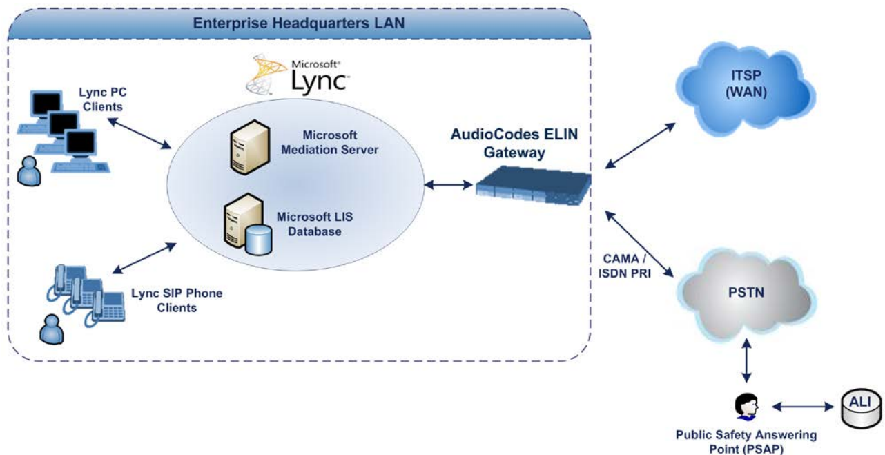
Figure 25-8: AudioCodes ELIN Gateway for E9-1-1 in Lync Server 2010 Environment
