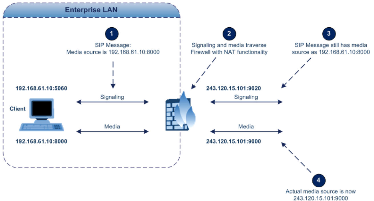
Figure 11-12: Device behind NAT and NAT Issues
