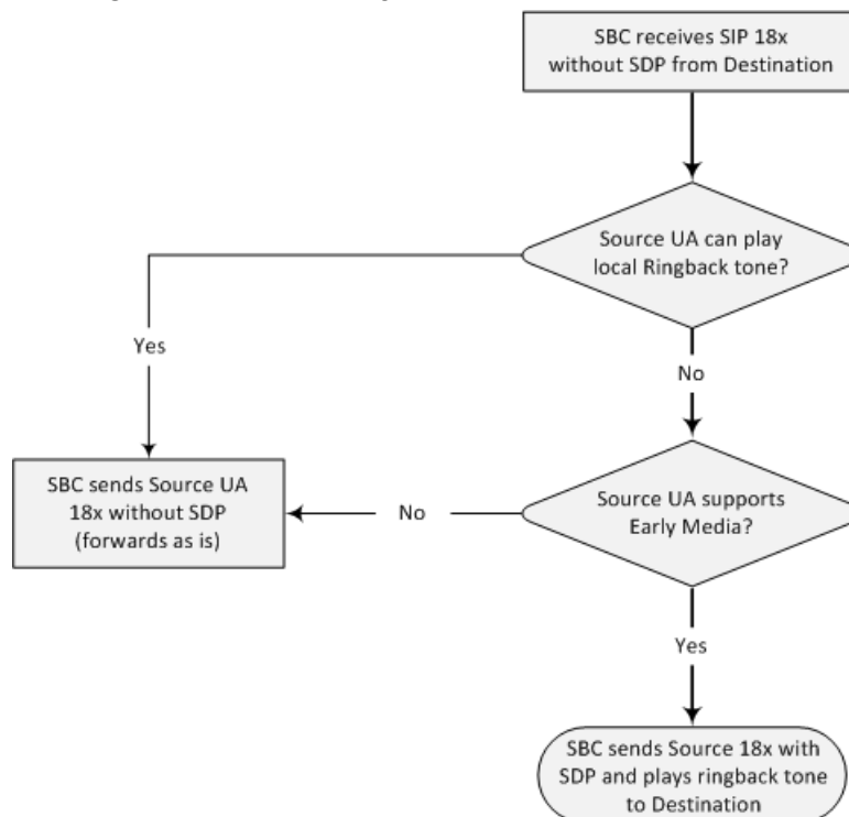
Figure 27-7: SBC Early Media RTP 18x without SDP
