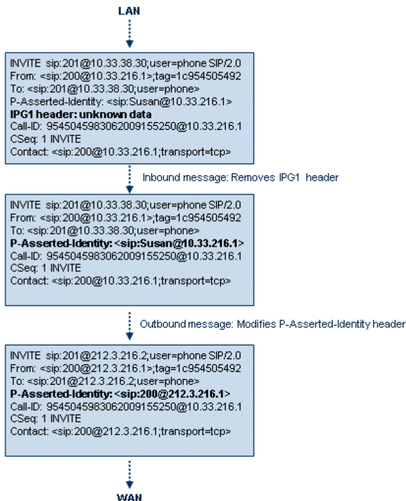
Figure 17-1: SIP Header Manipulation Example
