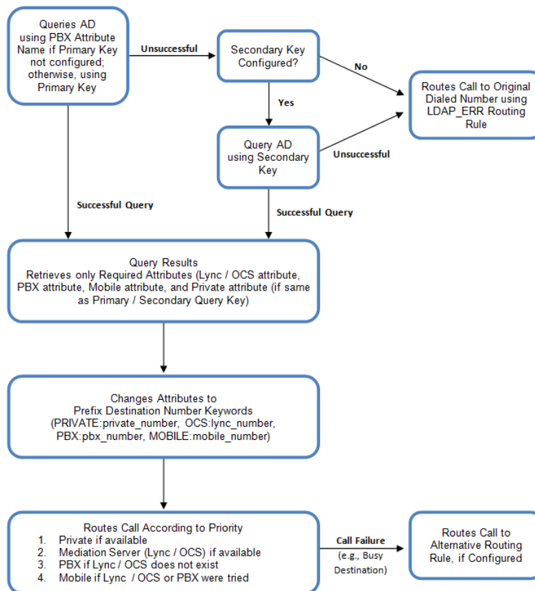
Figure 14-4: LDAP Query Flowchart
