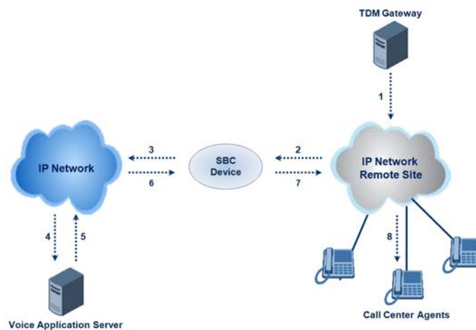
Figure 27-11: Normal Operation in Call Center Application
