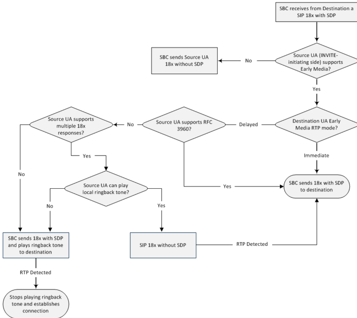
Figure 27-8: Early Media RTP - SIP 18x with SDP
