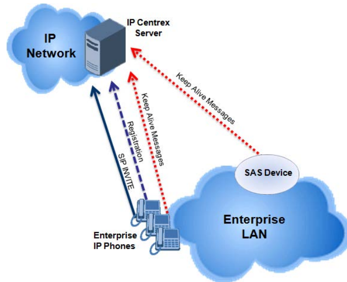
Figure 31-3: SAS Redundant Mode in Normal State (Example)
