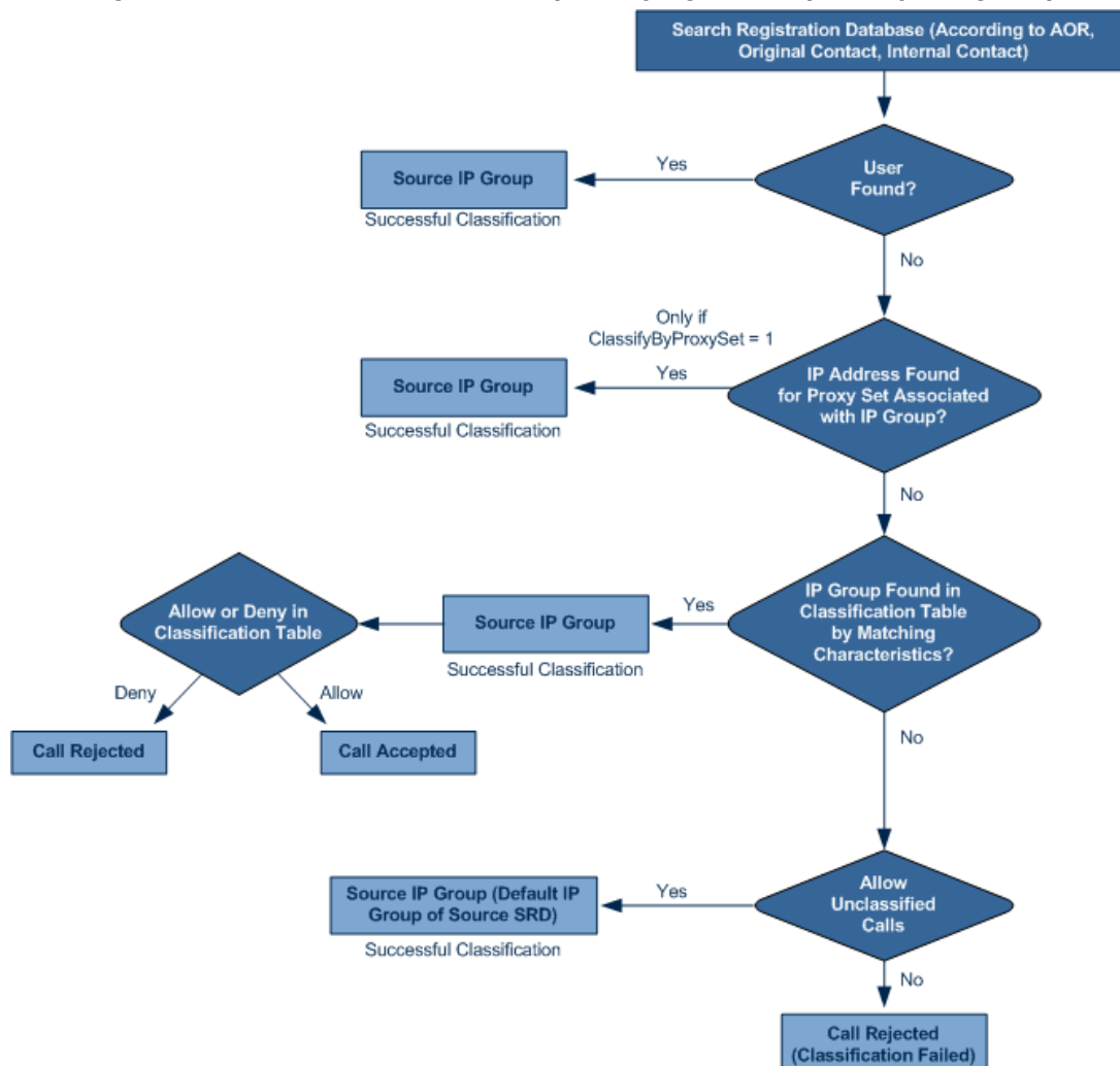
Figure 28-4: Classification Process (Identifying IP Group or Rejecting Call)
