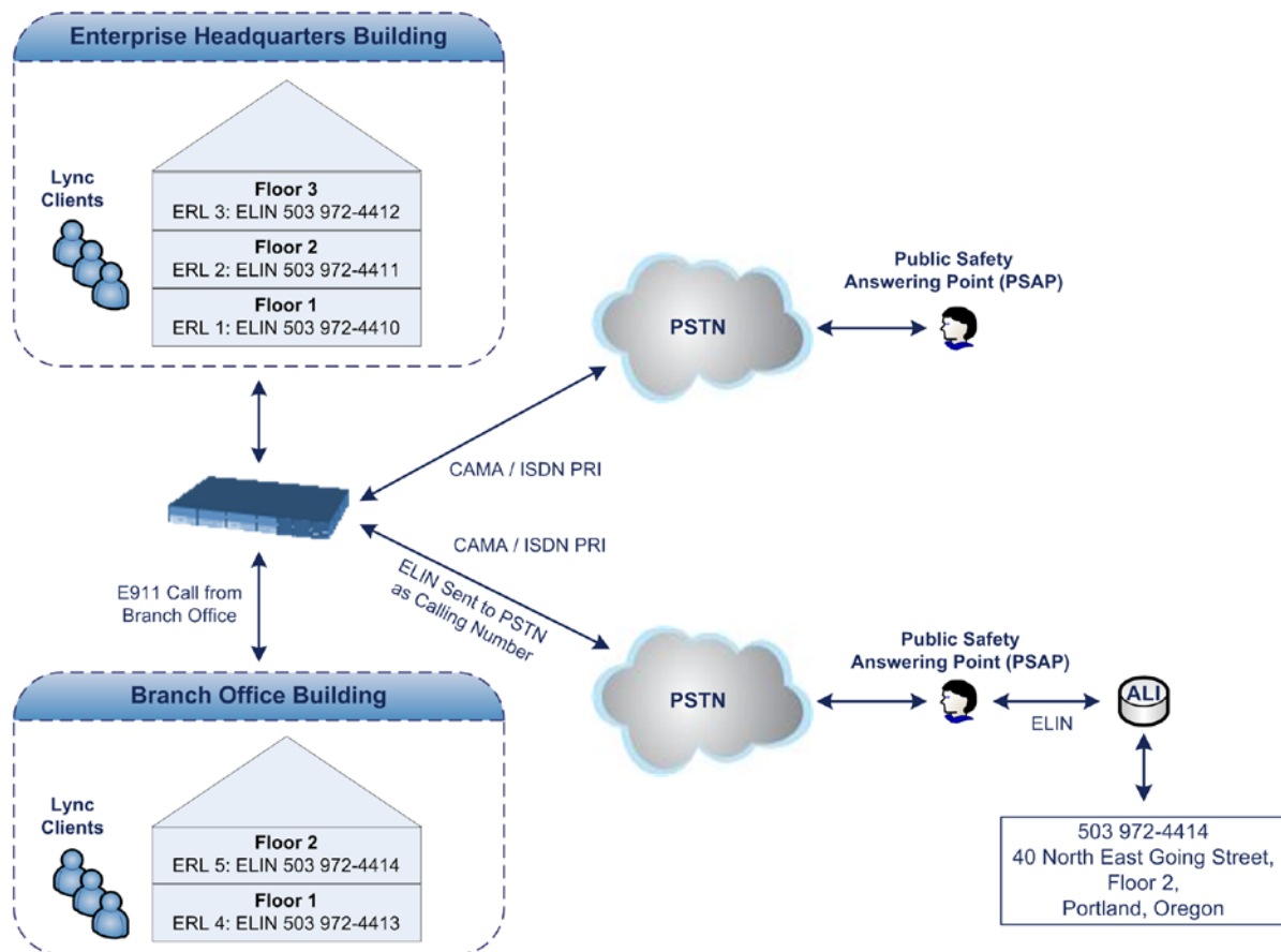
Figure 25-7: Implementing ERLs and ELINs for E9-1-1 in Lync Server 2010
