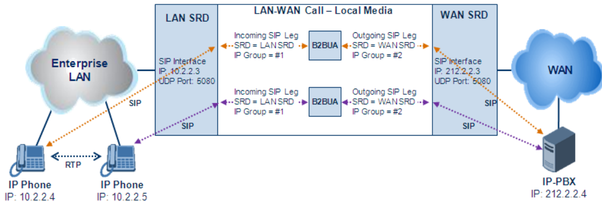
Figure 27-5: SBC SIP Signaling without RTP Media Flow
