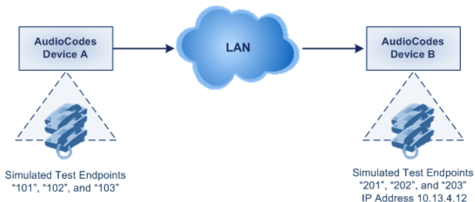
Figure 52-9: Batch Test Call Example
