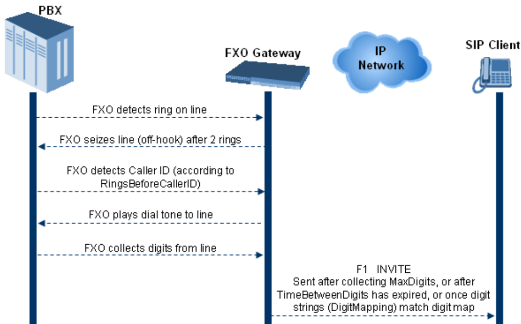
Figure 26-14: Call Flow for Collecting Digits Mode
