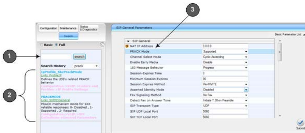
Figure 4-15: Searched Result Screen
