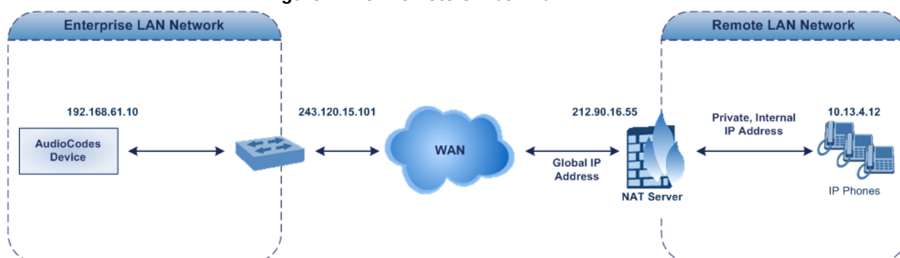
Figure 11-15: Remote UA behind NAT
