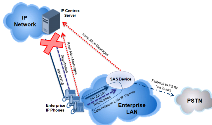
Figure 31-4: SAS Redundant Mode in Emergency State (Example)
