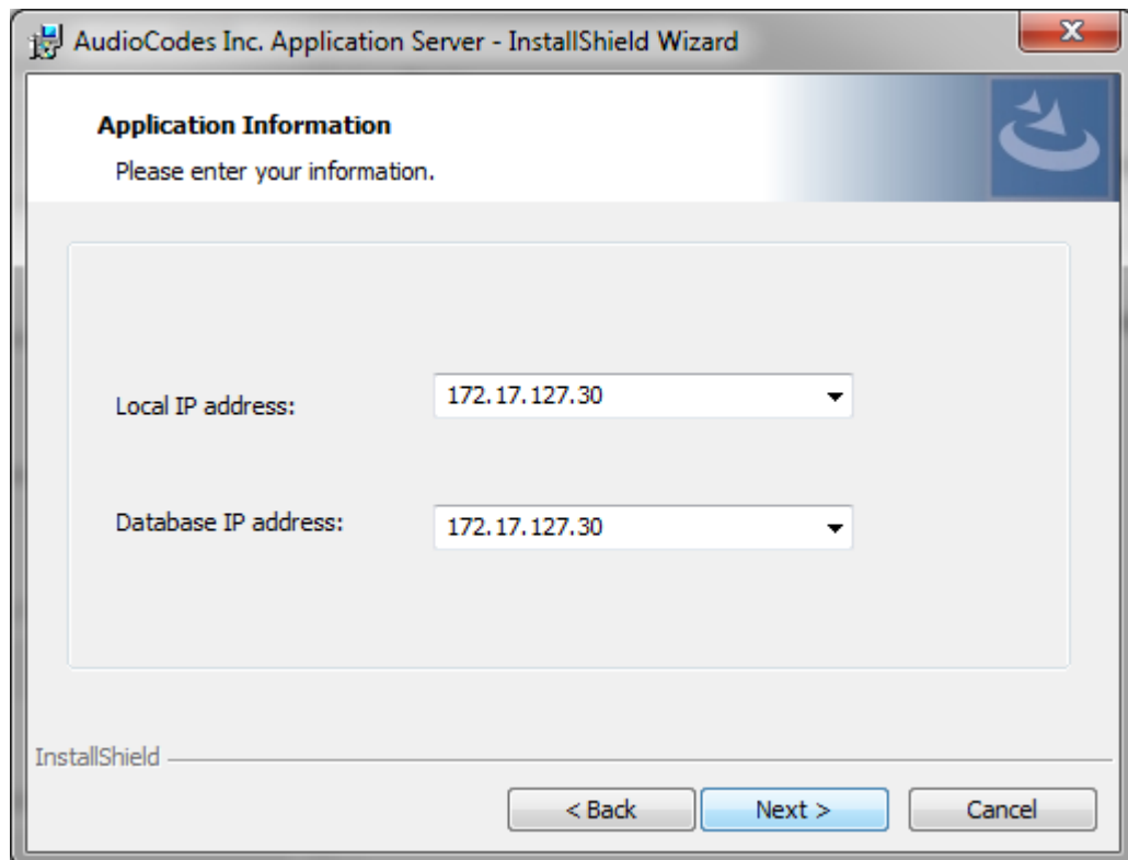
Figure 4-8: Application Information
