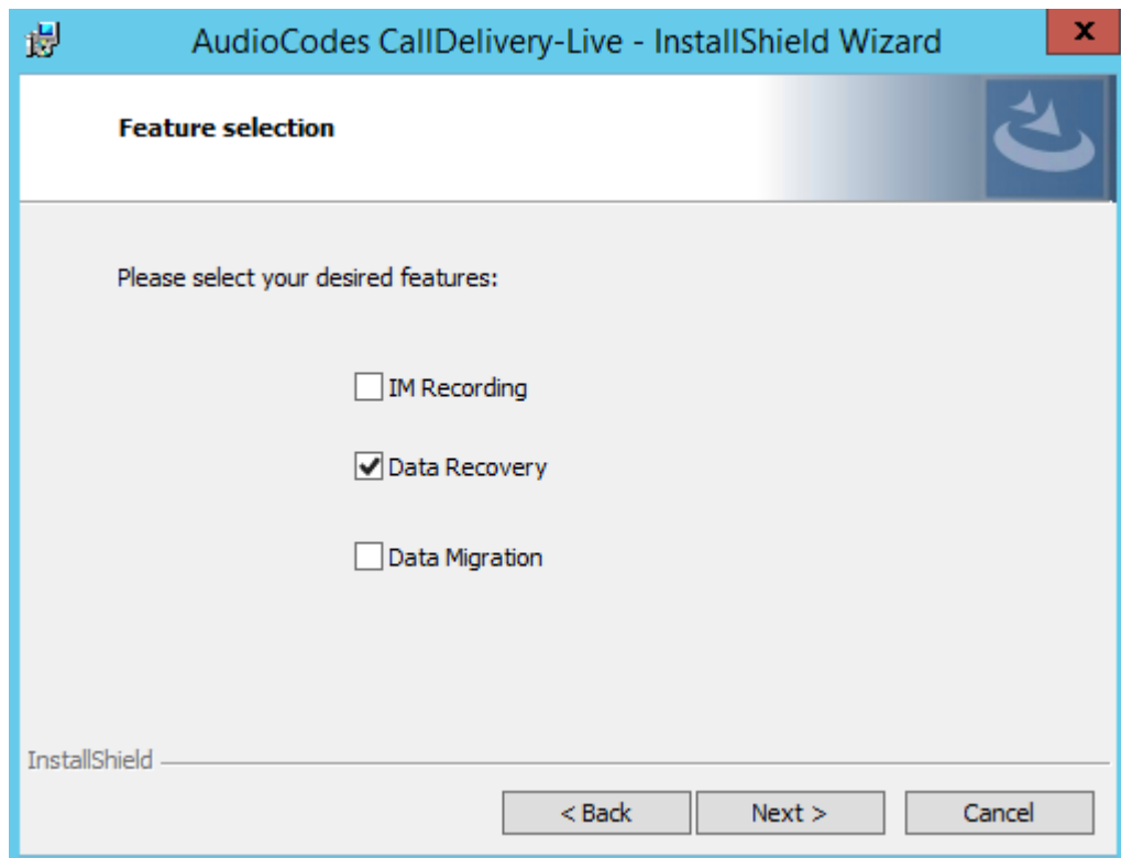
Figure 5-22: Setup Type
