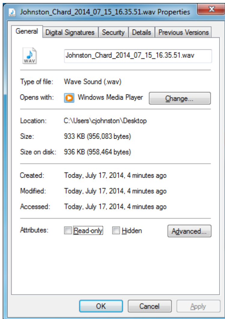
Figure 10-1: Digital Signatures
