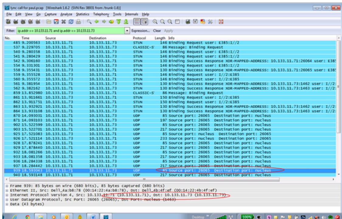
Figure 12-4: Sniffer Trace
