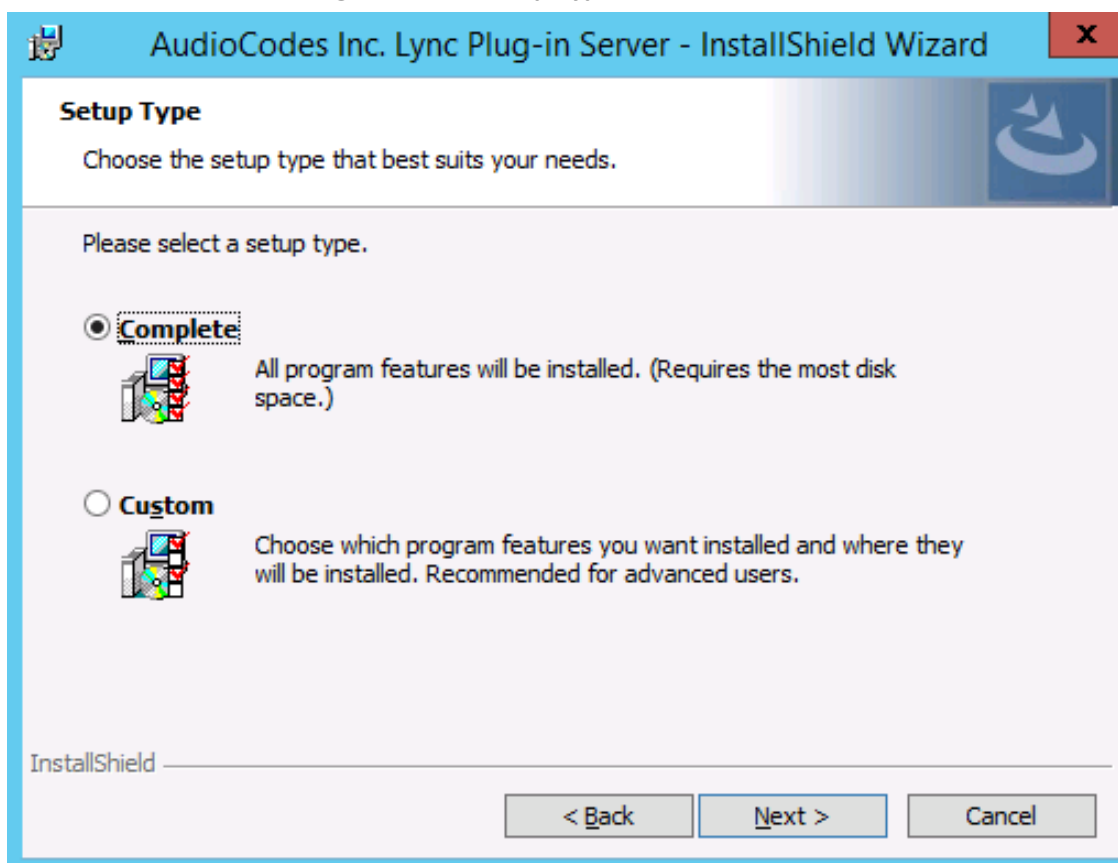
Figure 8-31: Setup Type
