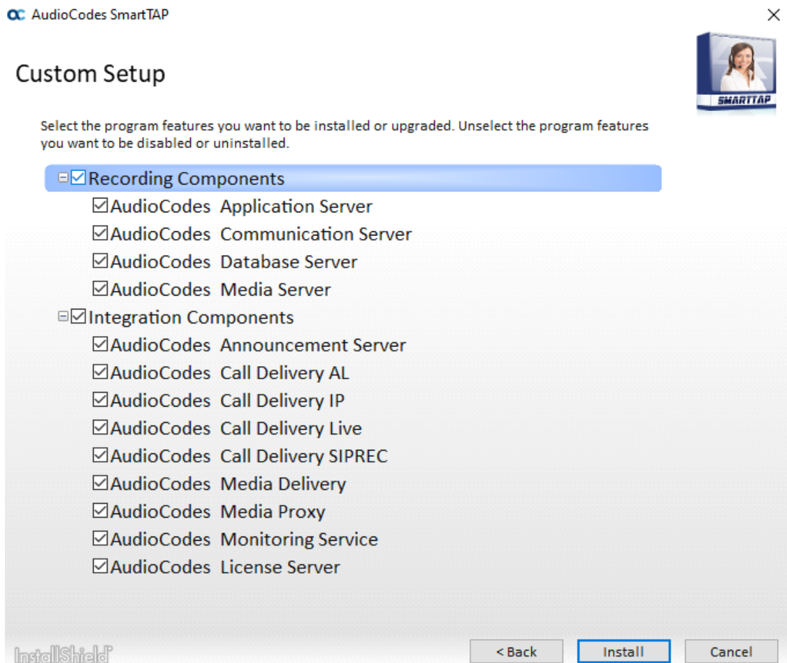
Figure 5-3: Custom Setup
