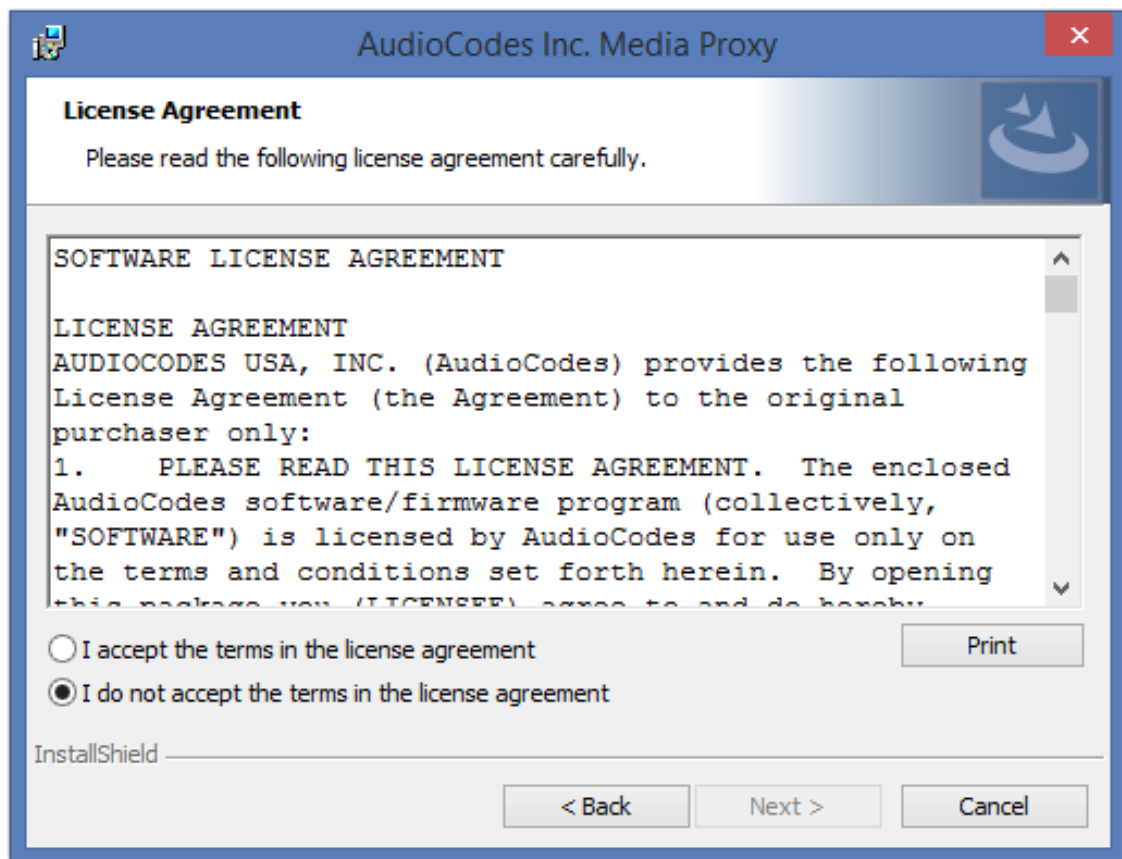
Figure 8-51: License Agreement
