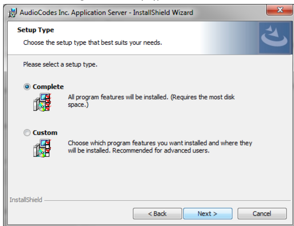
Figure 4-9: Setup Type
