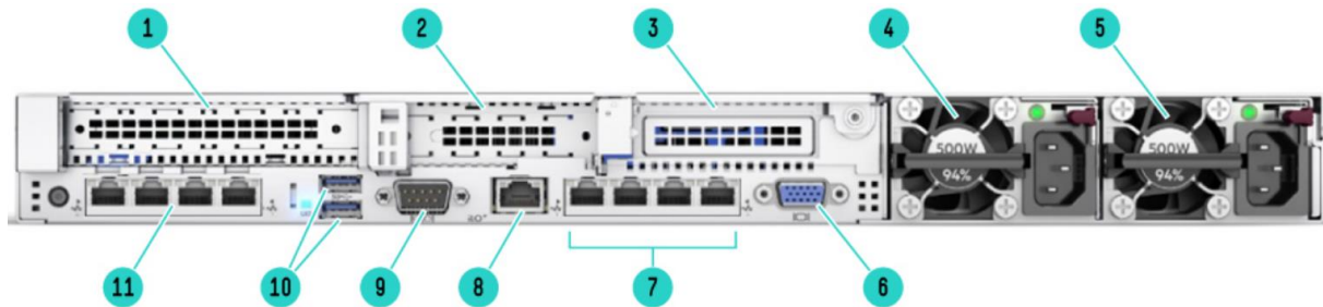
Figure 2-1: Rear Panel of HPE ProLiant DL360 Gen10
