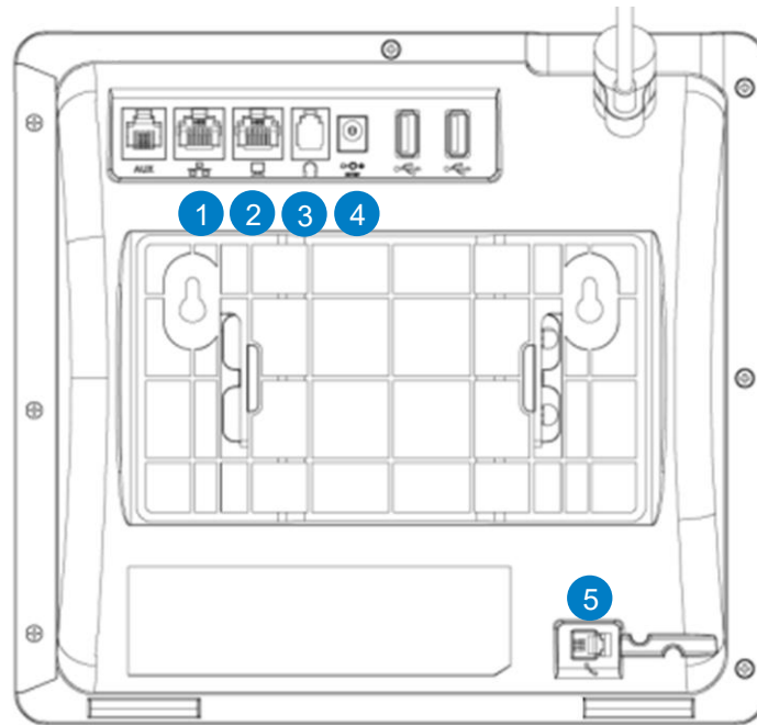
Figure 2: Rear View
