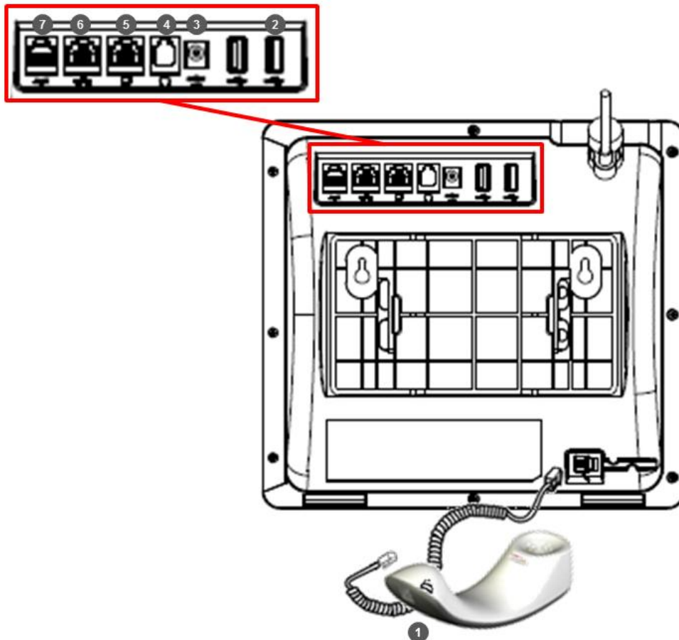
Figure 3: Cabling
